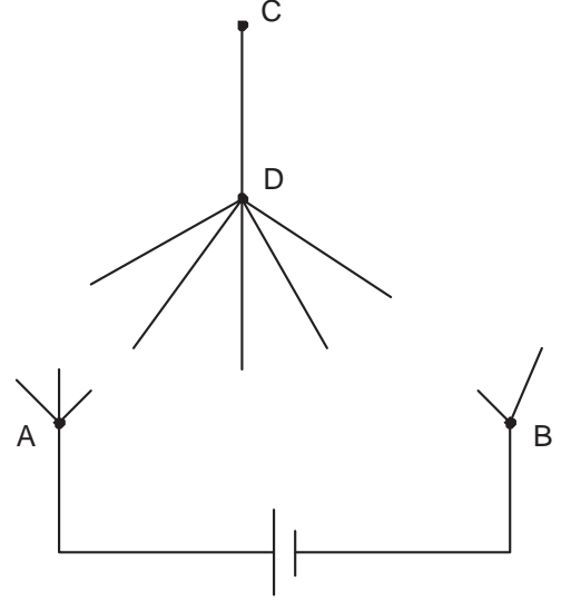
FIG. 2: A node with degree 1.
